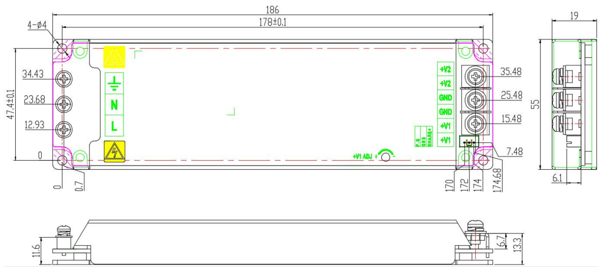
Dimensions and mounting holes - terminal coordinates
